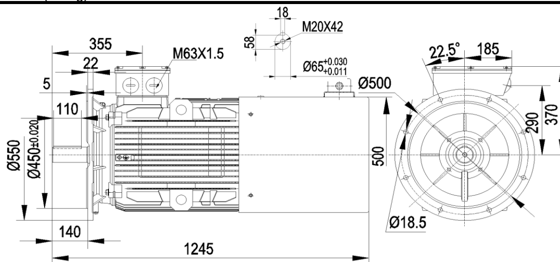
YEB4-280S 75kW(796kg)
