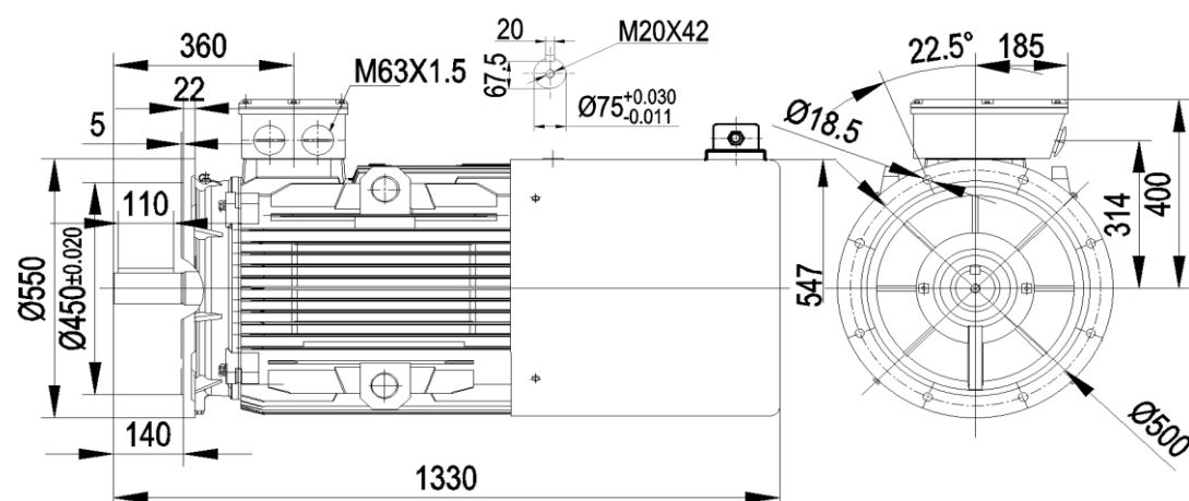
YEB4-280S 75kW(796kg)
