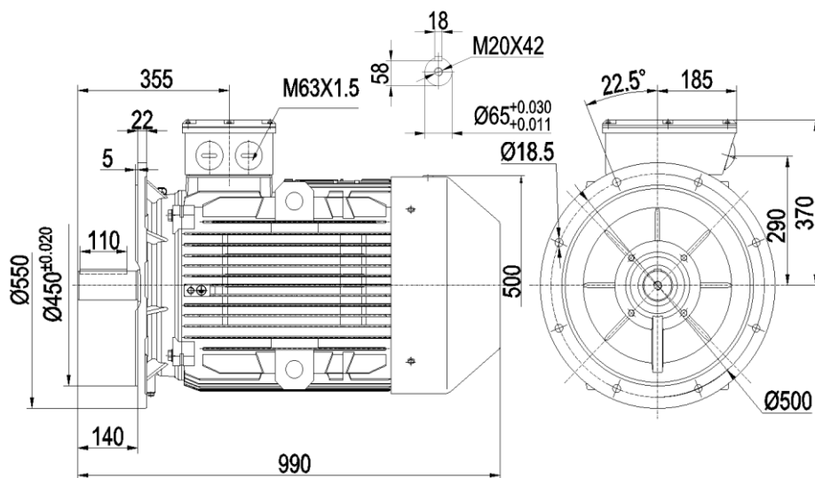
YE4-280S 75kW(700kg)
