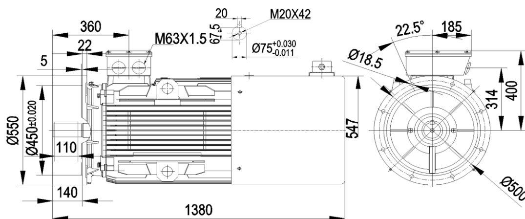
YEB4-280M 90kW(846kg)
