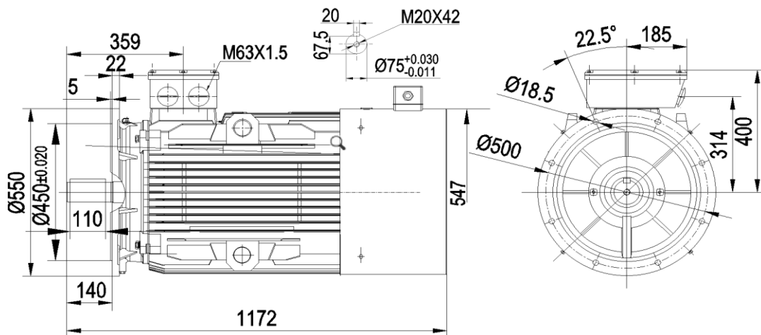
YE4-280M 90kW(750kg)
