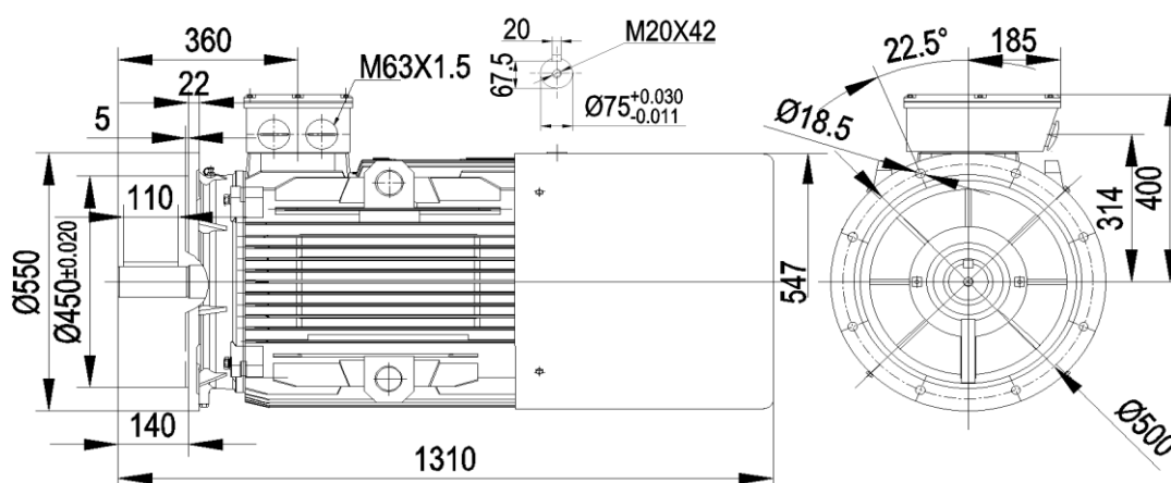
YEB4-280S 75kW(796kg)
