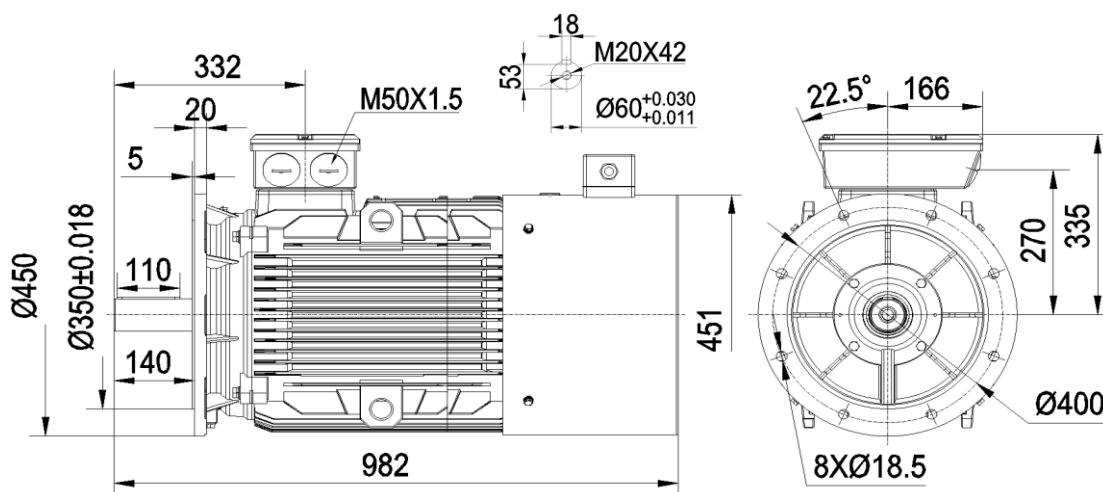
YE4-225M 45kW(425kg)
