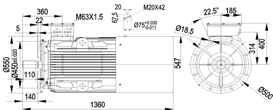
YEB4-280M 90kW(846kg)
